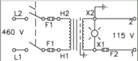
Schematic Standard w/Grounded Secondary without Receptacle
