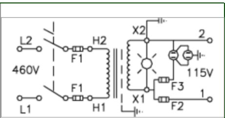
Schematic Standard w/Grounded Secondary with Receptacle
